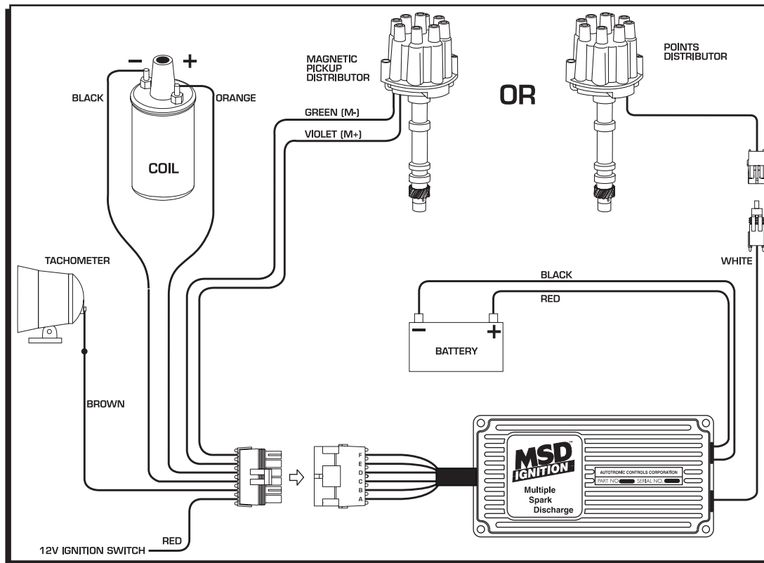
Figure 2 General Installation.
